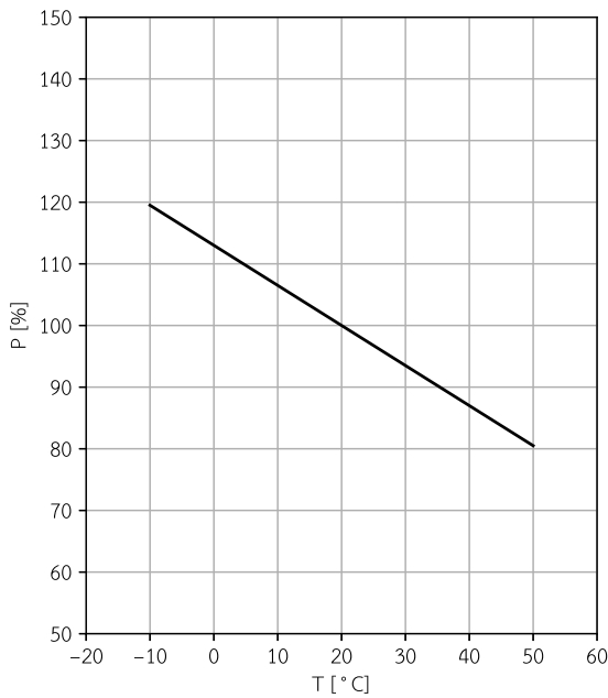
LWPRO-520-80 Relative output power vs. case temperature
