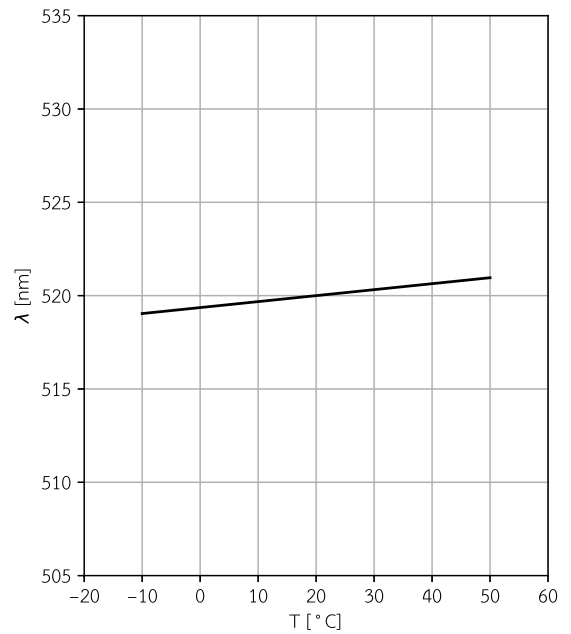
LWPRO-520-80 Wavelength vs. case temperature
