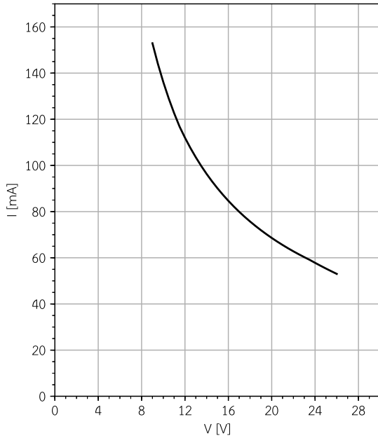
LWPRO-520-80 Input current vs. input voltage
