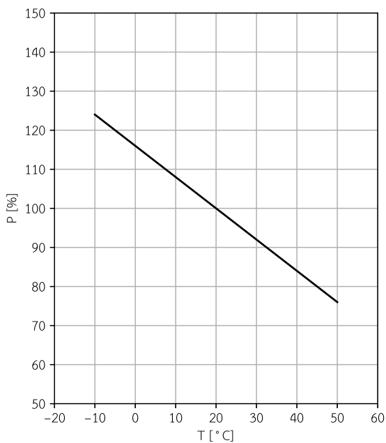
LWPRO-520-50 Relative output power vs. case temperature
