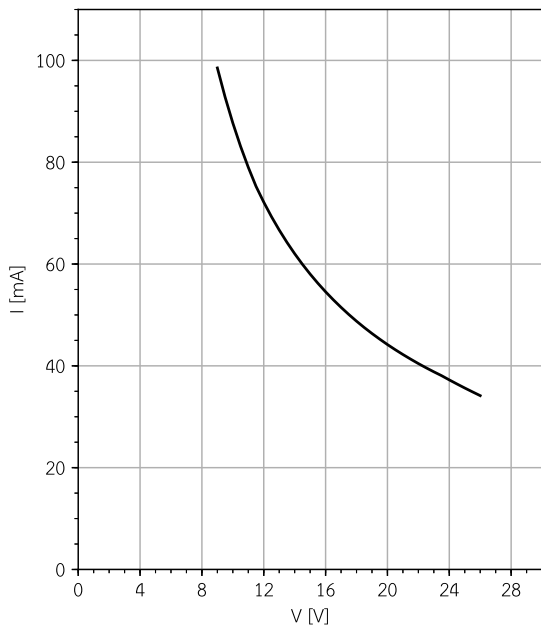
LWPRO-520-50 Input current vs. input voltage
