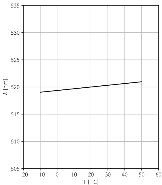
LWPRO-520-50 Wavelength vs. case temperature
