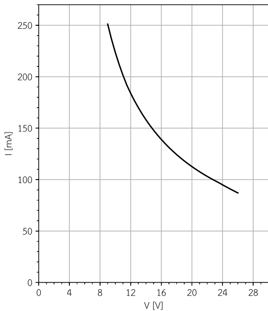
LWPRO-520-180 Input current vs. input voltage
