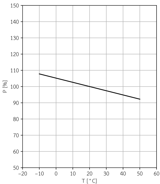
LWPRO-520-180 Relative output power vs. case temperature
