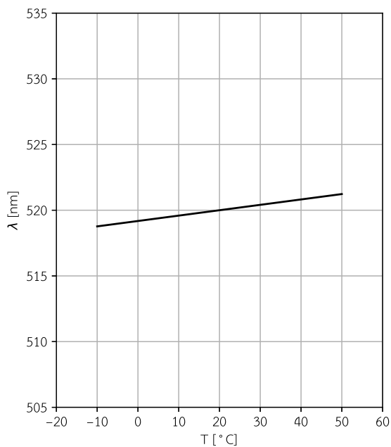
LWPRO-520-180 Wavelength vs. case temperature
