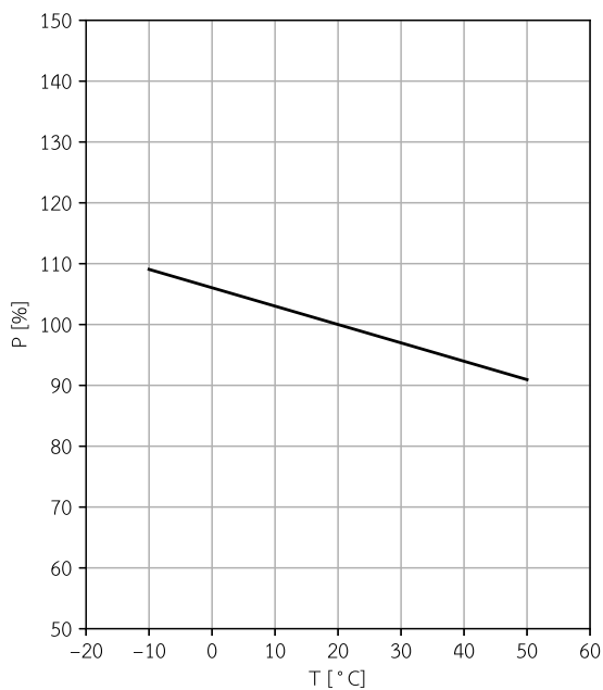
LWPRO-520-130 Relative output power vs. case temperature
