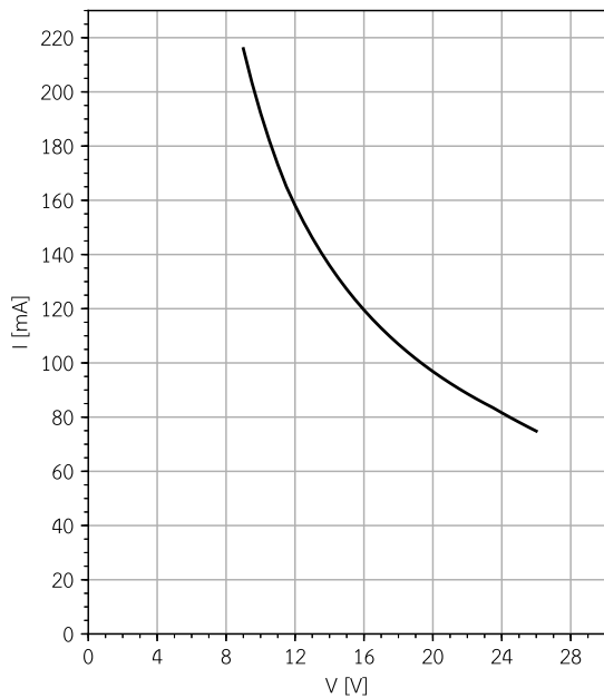
LWPRO-520-130 Input current vs. input voltage
