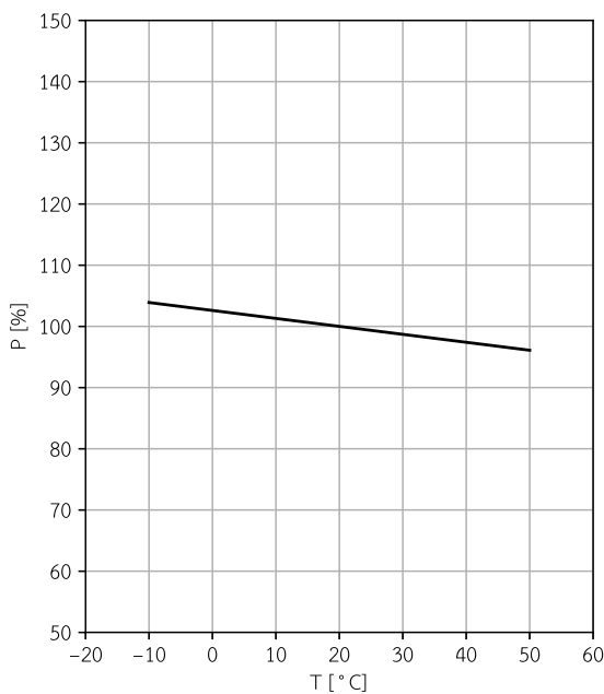
Relative output power vs. case temperature
