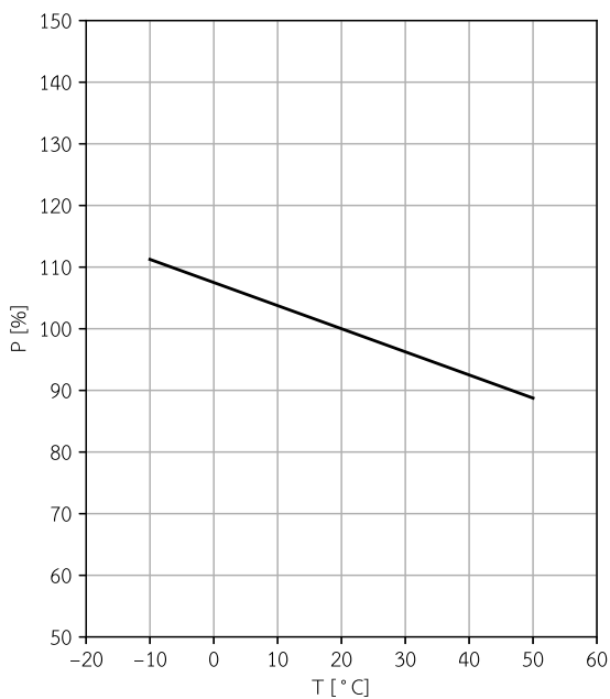
LW-850-50-C12-DI Relative output power vs. case temperature
