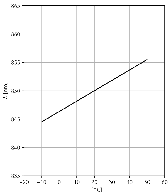
LW-850-50-C12-DI Wavelength vs. case temperature
