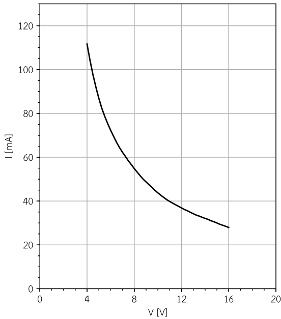
LW-785-120-C12-DM Input current vs. input voltage
