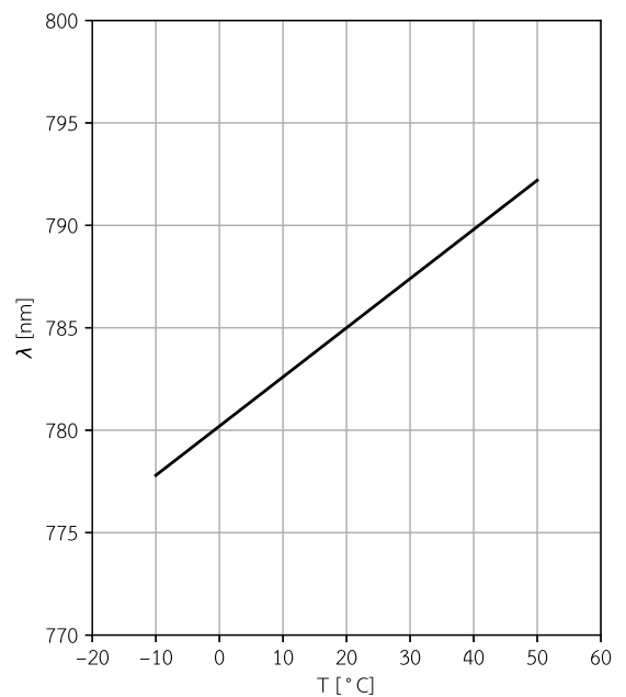
LW-785-120-C12-DM Wavelength vs. case temperature
