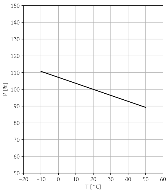
LW-785-120-C12-DM Relative output power vs. case temperature
