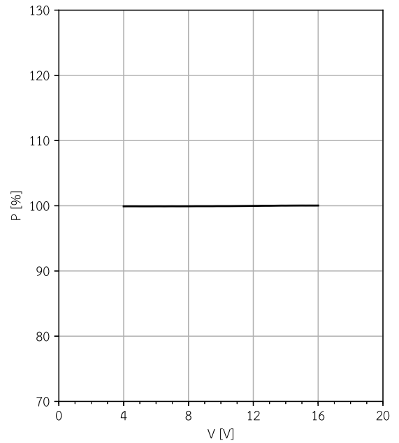
LW-785-120-C12-DM Relative output power vs. input voltage
