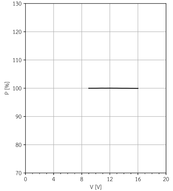
LW-520-80-C12-DM Relative output power vs. input voltage
