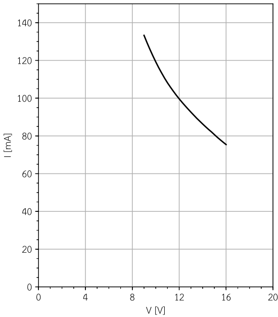
LW-520-80-C12-DM Input current vs. input voltage
