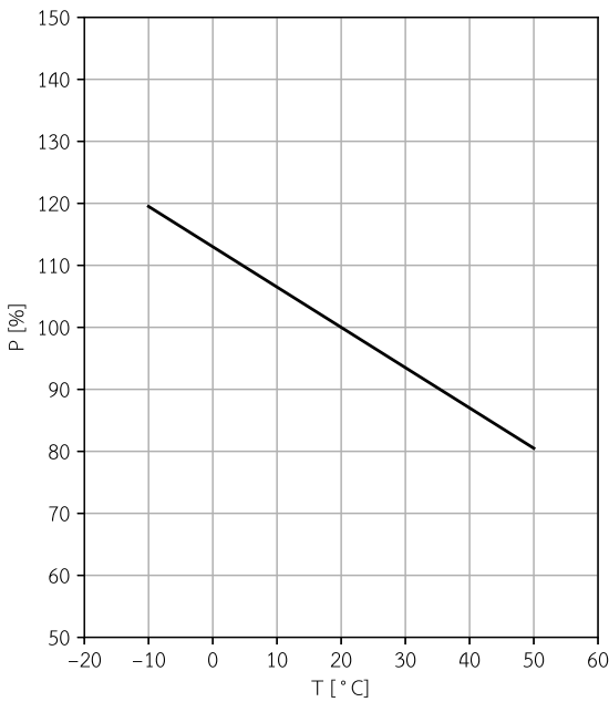
LW-520-80-C12-DM Relative output power vs. case temperature
