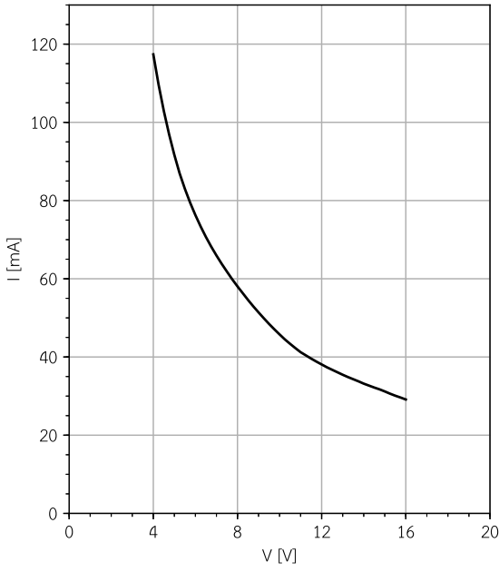
LW-505-30-C12-DI Input current vs. input voltage
