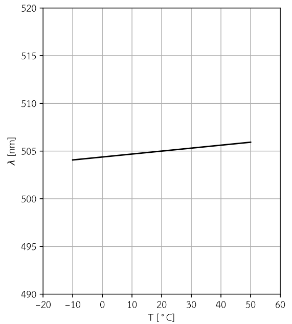
LW-505-30-C12-DI Wavelength vs. case temperature
