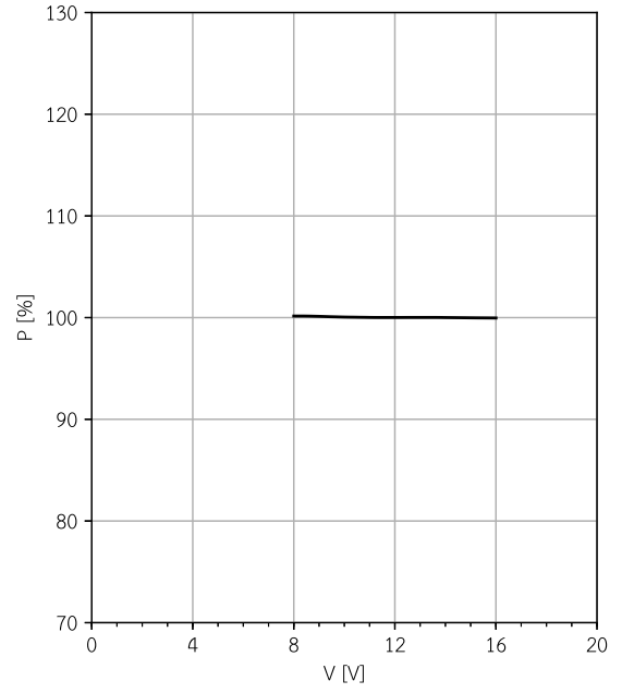
LW-405-500-C16-DM Relative output power vs. input voltage
