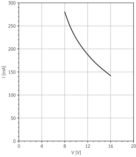
LW-405-500-C16-DM Input current vs. input voltage
