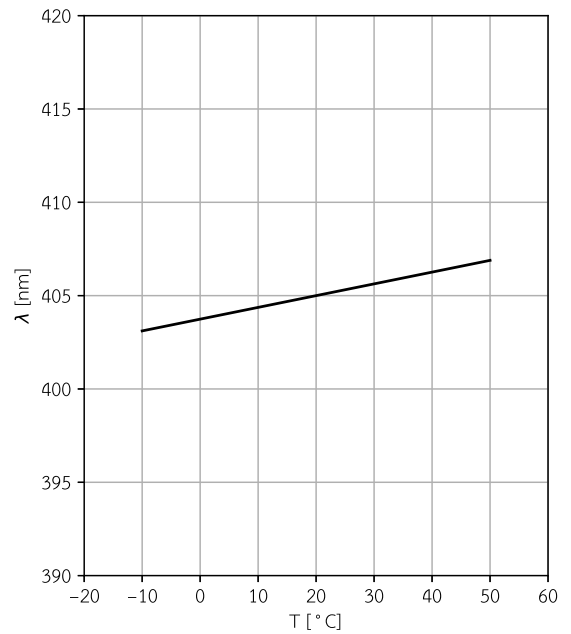
LW-405-150-C12-DM Wavelength vs. case temperature
