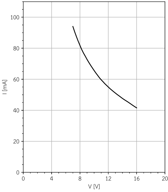
LW-405-150-C12-DM Input current vs. input voltage
