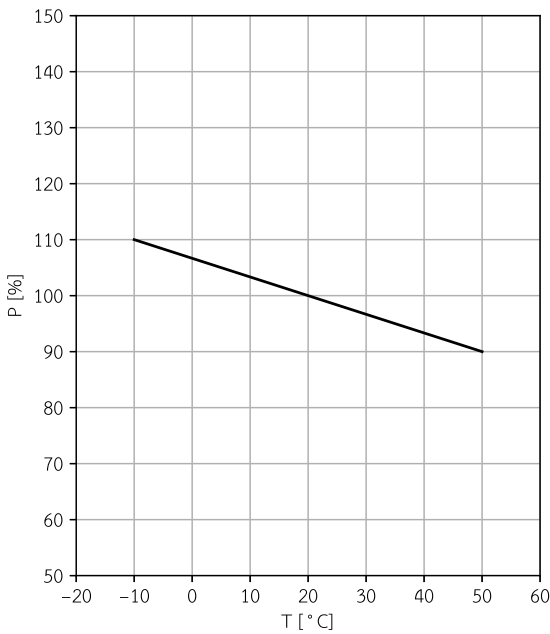
LW-405-150-C12-DM Relative output power vs. case temperature
