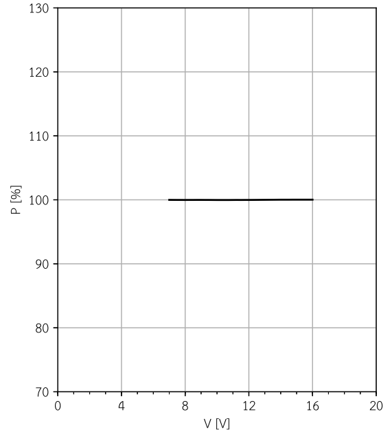
LW-405-150-C12-DM Relative output power vs. input voltage
